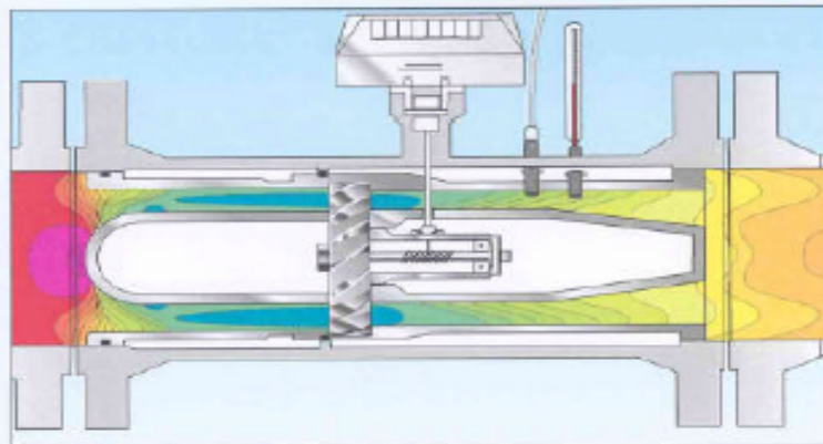
Change of temperature within the gas flow
